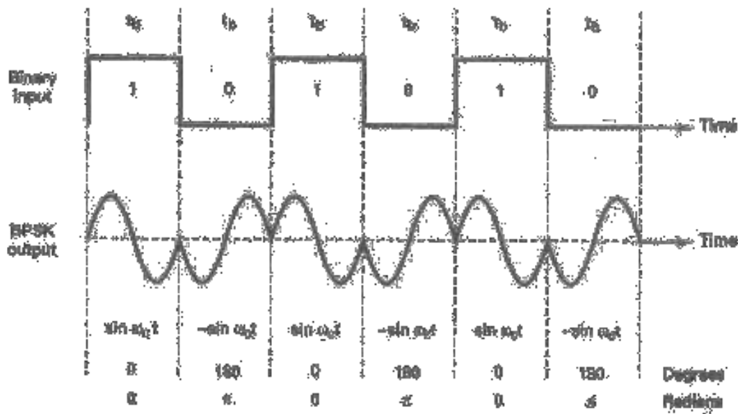
FIGURE 9-10 Output phase versus time relationship for a BPSK modulator.
