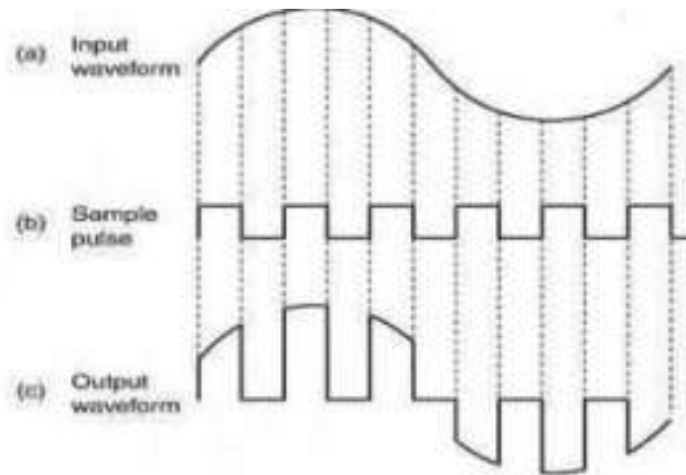
Natural sampling
