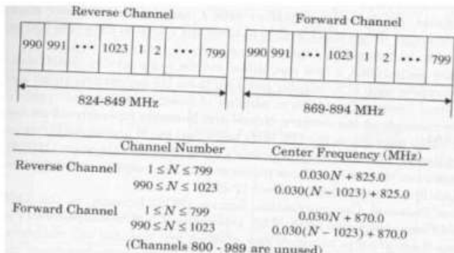
Complete AMPS Frequency spectrum
