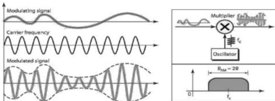
AM generation
