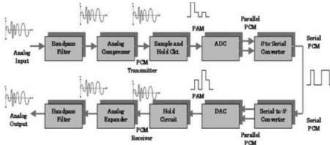
PCM system with analog companding
