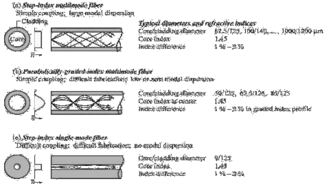
Fig. 12.1. (a) Step-index multimode fibers allow for the propagation of several optical modes. (b) Parabolically graded-index multimode fibers allow for the propagation of several modes with similar propagation constant. Graded-index multimode fibers have a lower modal dispersion than step-index multimode fibers. (c) Step-index single-mode fibers have a small core diameter and no modal dispersion.
