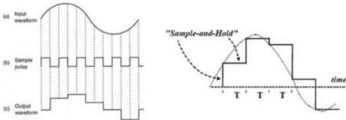
Flat-top sampling
