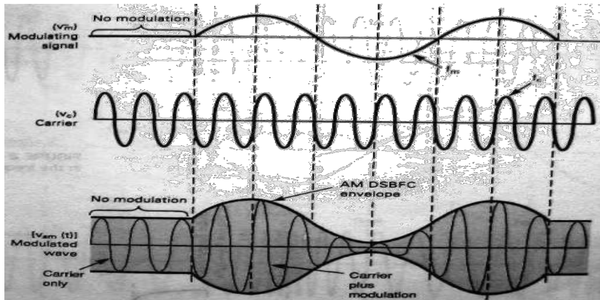
AM generation
