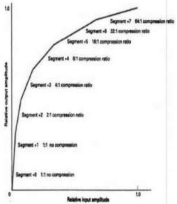
\mu - 255 compression characteristics
